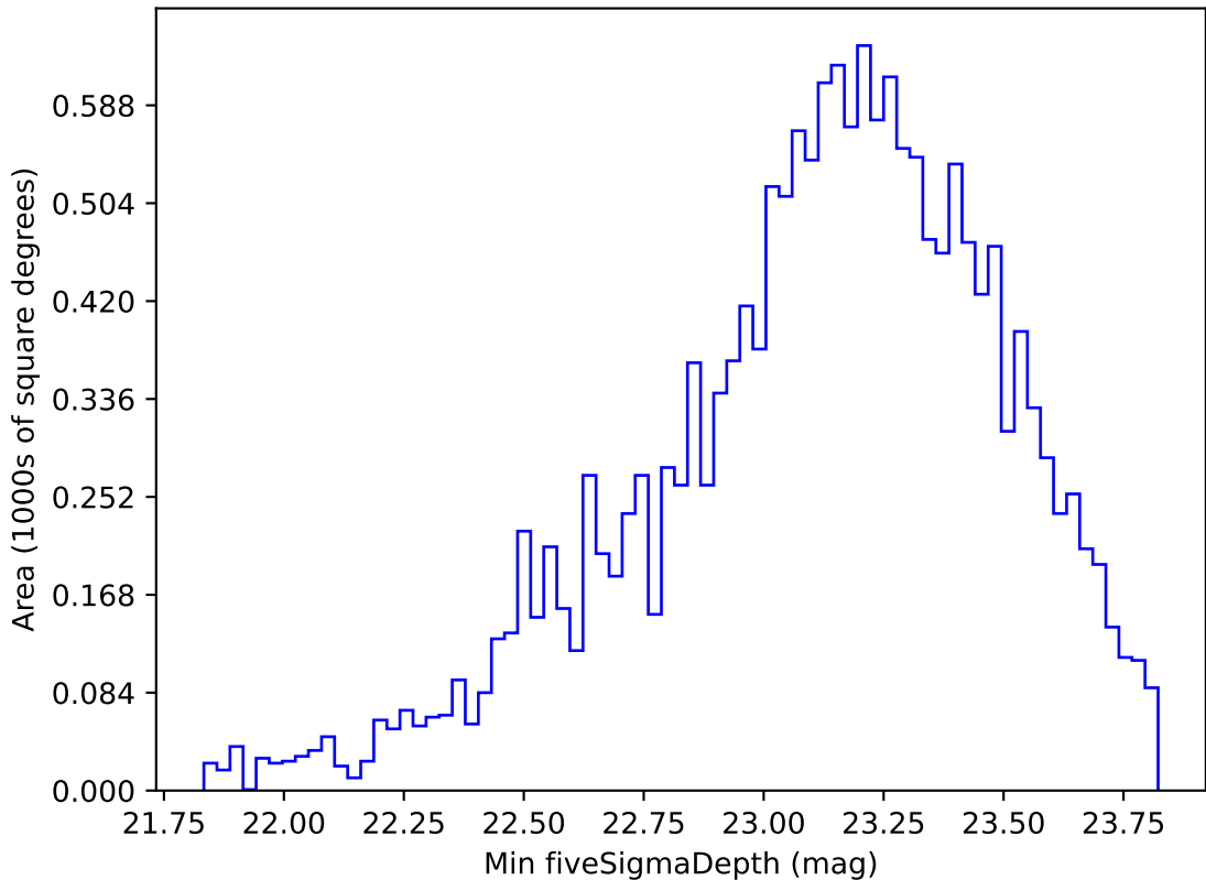
too_elab_r16_d2_griz_v3.4_10yrs WFD g band: Min fiveSigmaDepth
