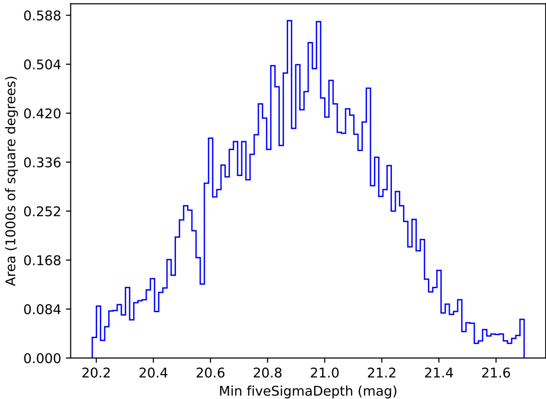
too_elab_r16_d2_griz_v3.4_10yrs All sky y band: Min fiveSigmaDepth
