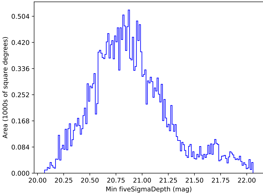
too_elab_r16_d2_griz_v3.4_10yrs All sky all bands: Min fiveSigmaDepth
