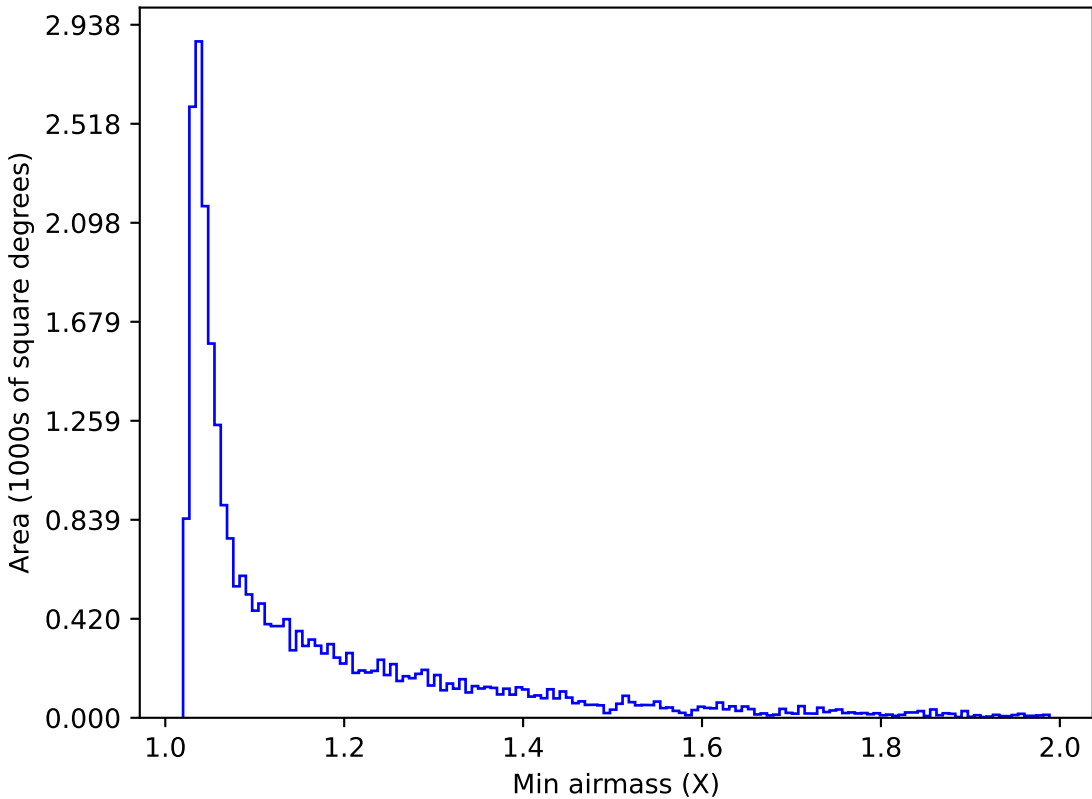
too_elab_r16_d2_griz_v3.4_10yrs Yr 1 r band: Min airmass
