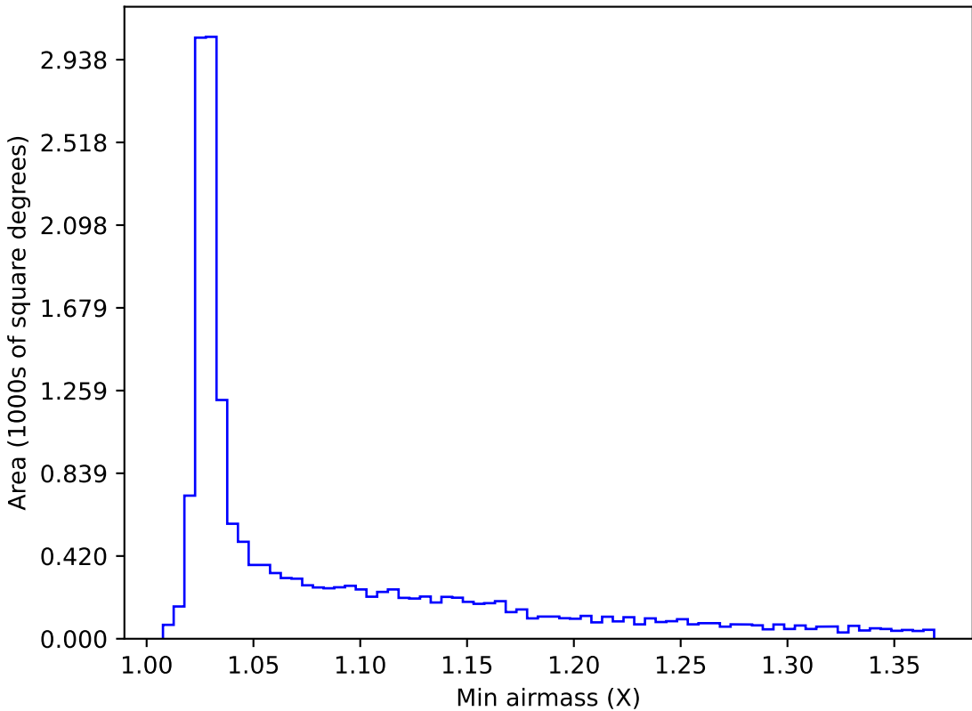
too_elab_r16_d2_griz_v3.4_10yrs WFD z band: Min airmass
