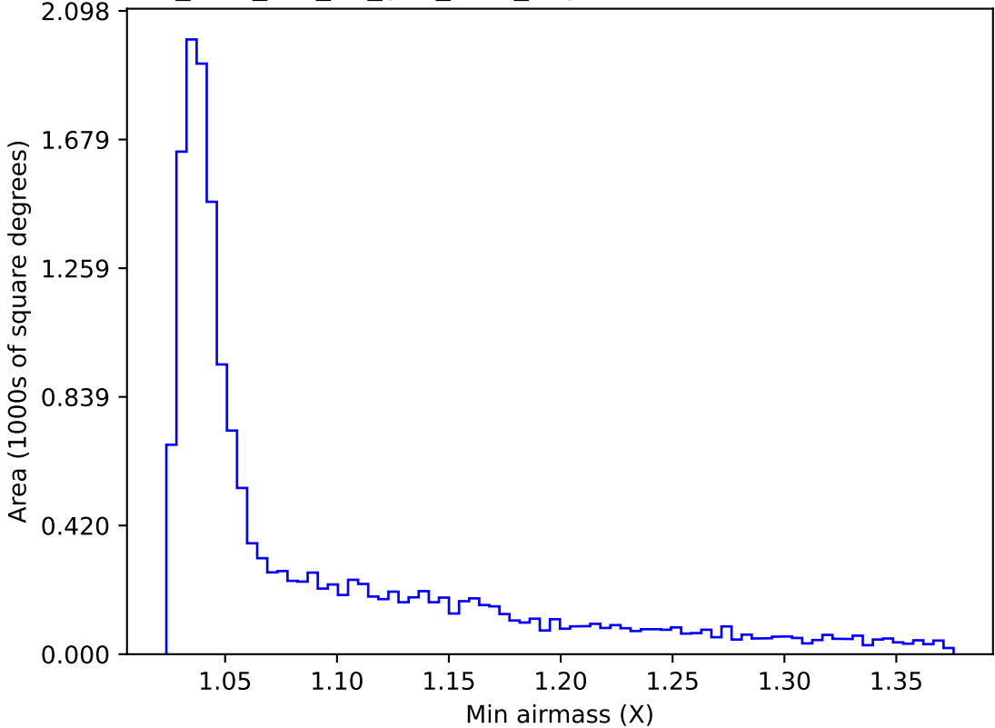
too_elab_r16_d2_griz_v3.4_10yrs WFD u band: Min airmass
