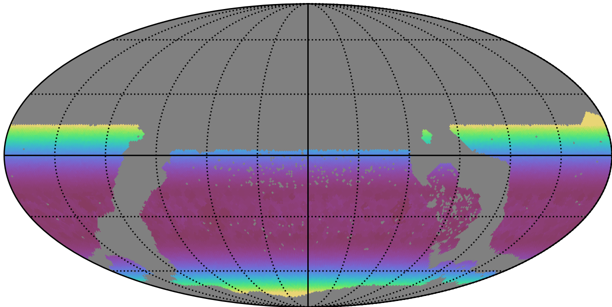
too_elab_r16_d2_griz_v3.4_10yrs WFD r band: Min airmass
