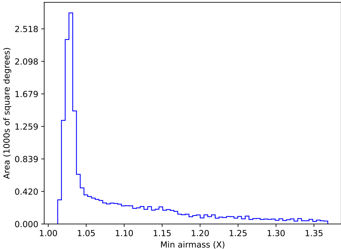
too_elab_r16_d2_griz_v3.4_10yrs WFD r band: Min airmass
