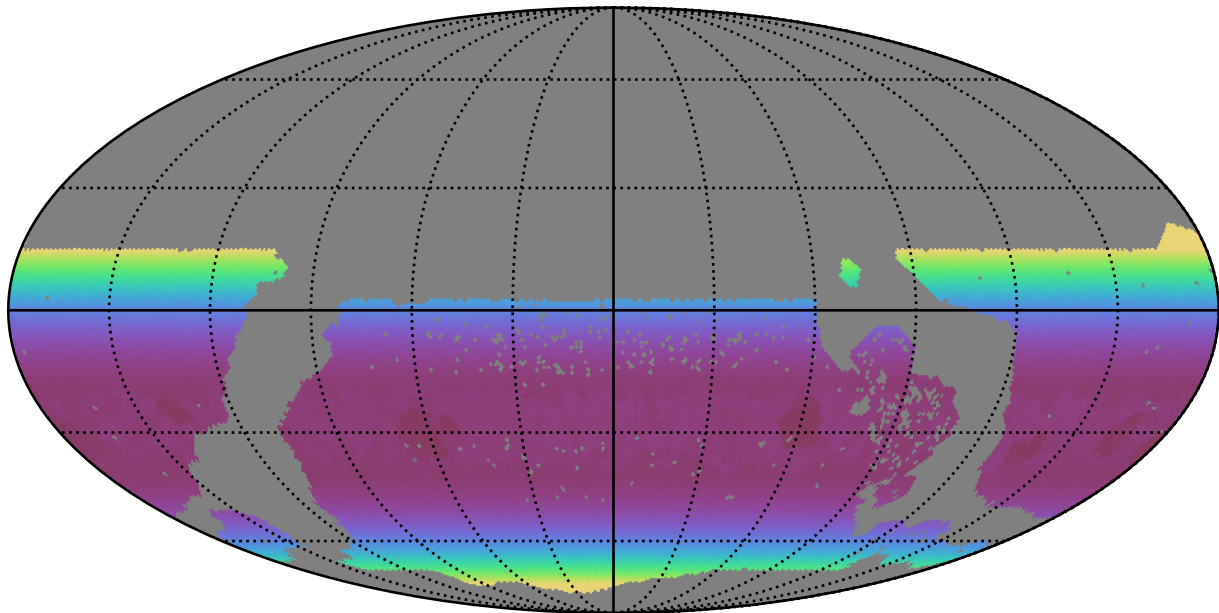
too_elab_r16_d2_griz_v3.4_10yrs WFD all bands: Min airmass
