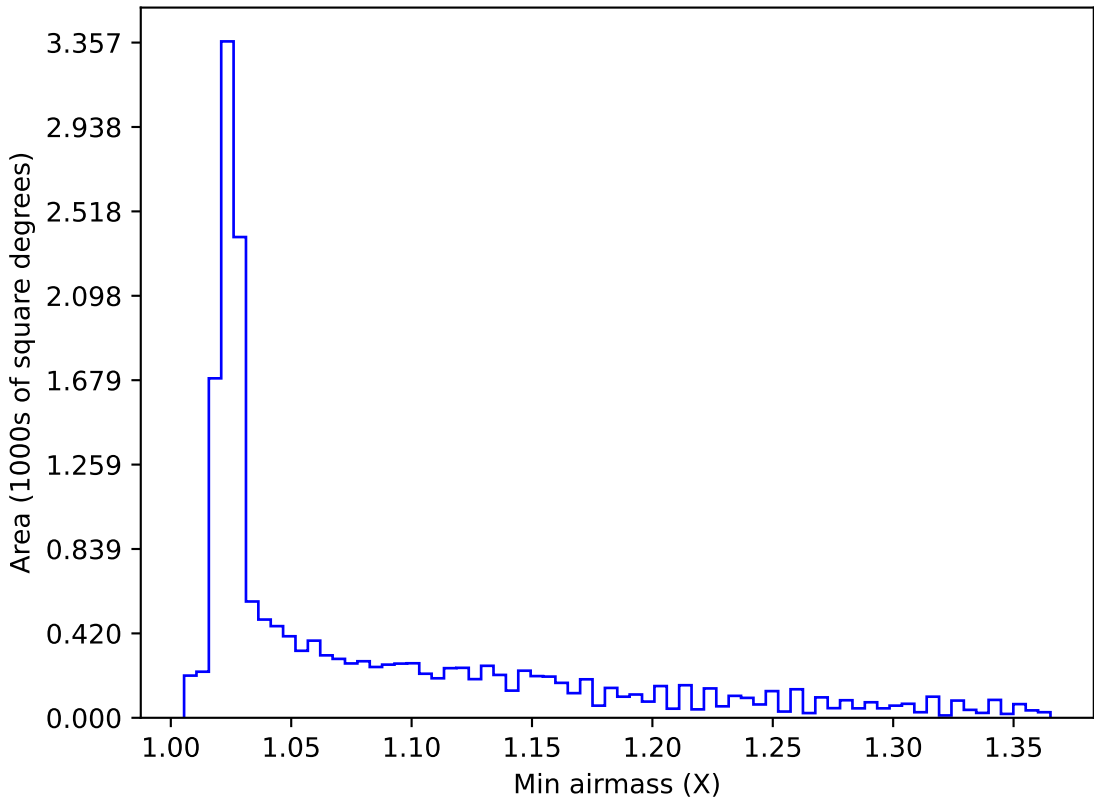
too_elab_r16_d2_griz_v3.4_10yrs WFD all bands: Min airmass
