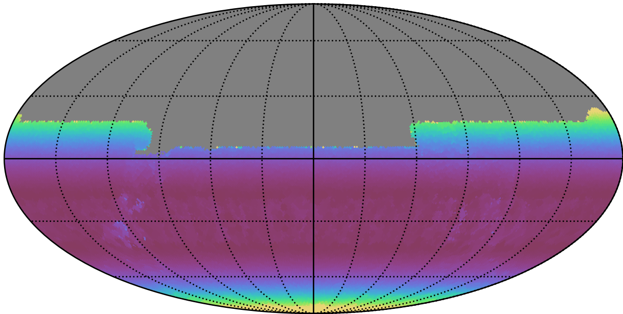
too_elab_r16_d2_griz_v3.4_10yrs All sky u band: Min airmass
