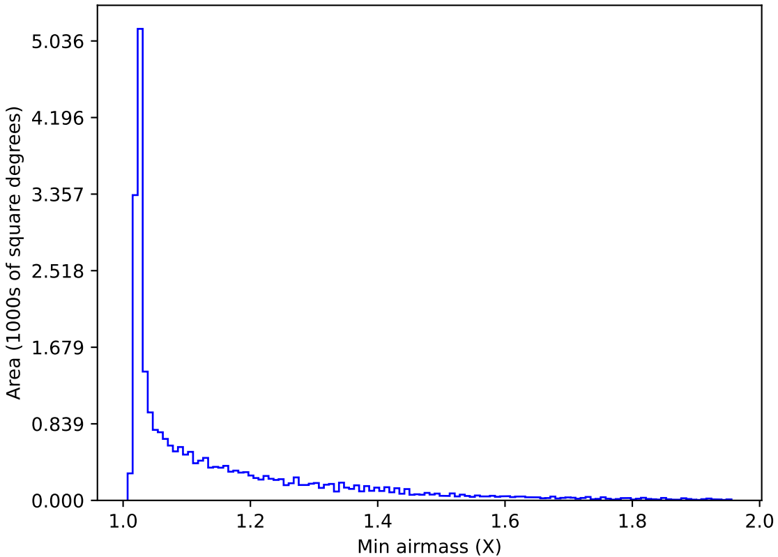
too_elab_r16_d2_griz_v3.4_10yrs All sky all bands: Min airmass
