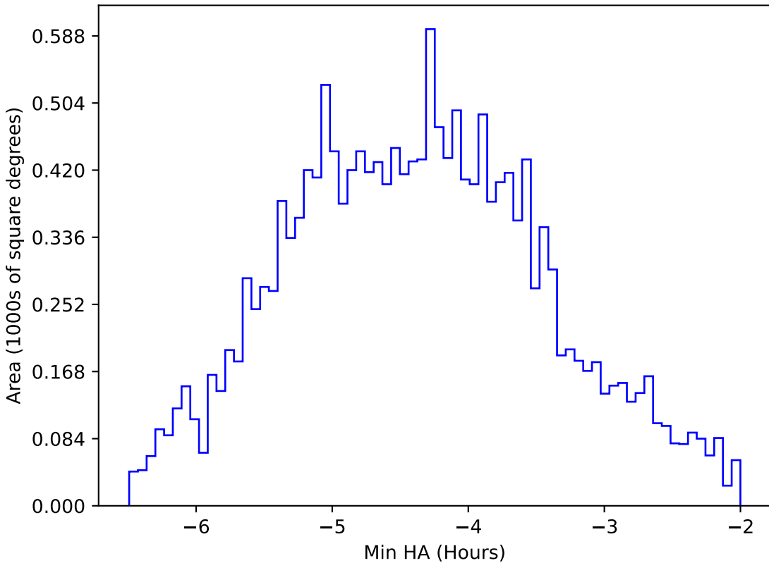
too_elab_r16_d2_griz_v3.4_10yrs WFD z band: Min HA
