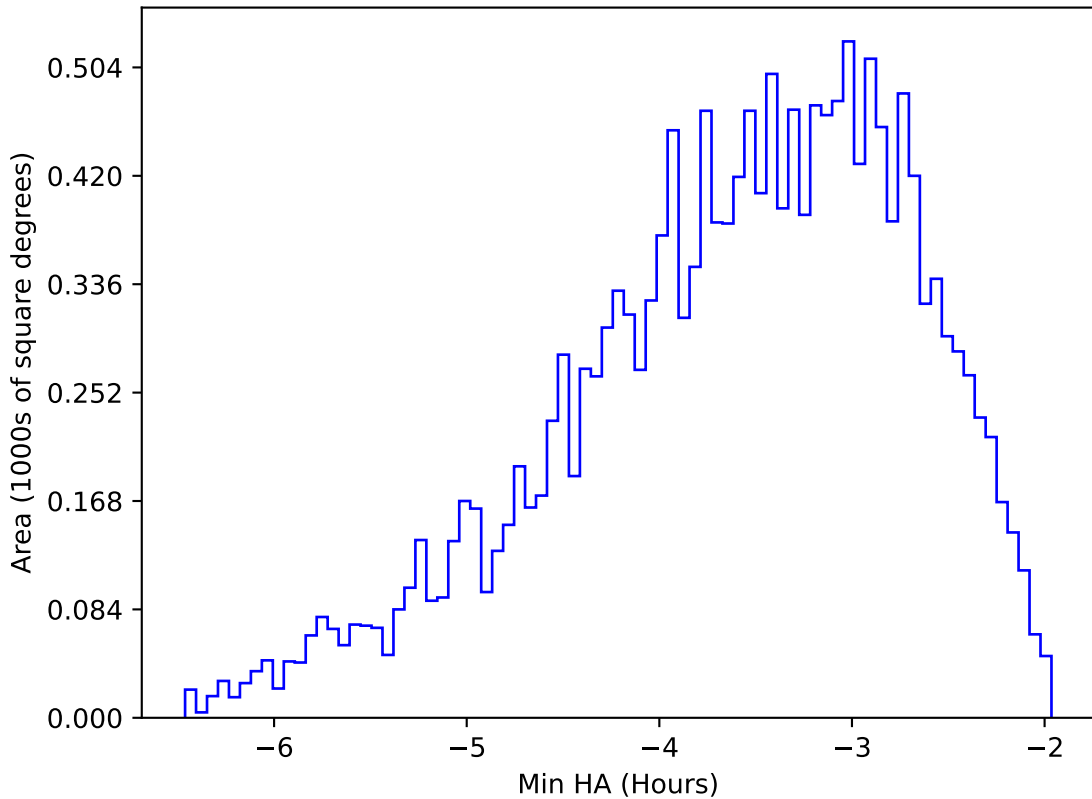
too_elab_r16_d2_griz_v3.4_10yrs WFD y band: Min HA
