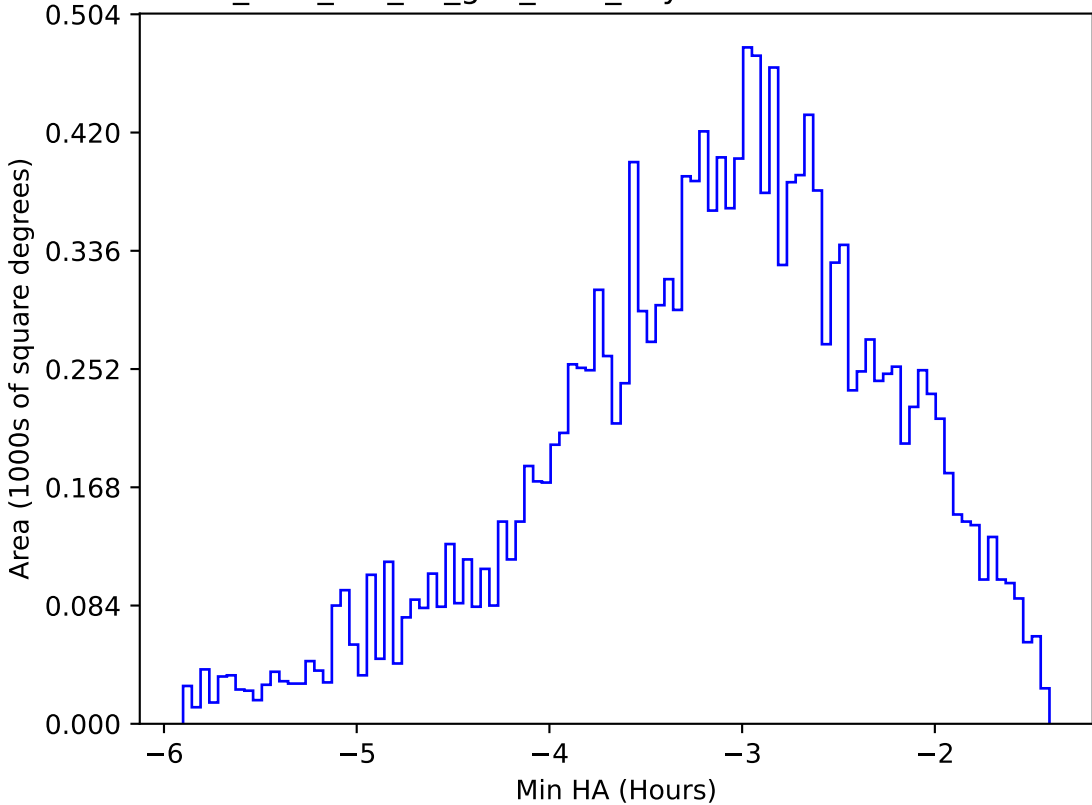
too_elab_r16_d2_griz_v3.4_10yrs WFD u band: Min HA
