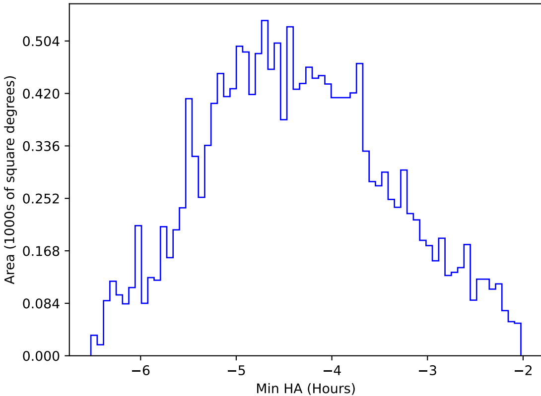
too_elab_r16_d2_griz_v3.4_10yrs WFD i band: Min HA
