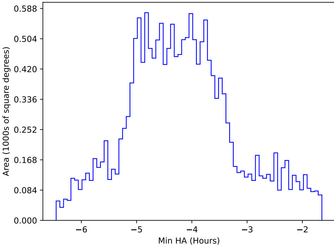
too_elab_r16_d2_griz_v3.4_10yrs WFD g band: Min HA
