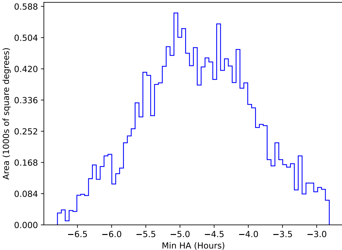
too_elab_r16_d2_griz_v3.4_10yrs WFD all bands: Min HA
