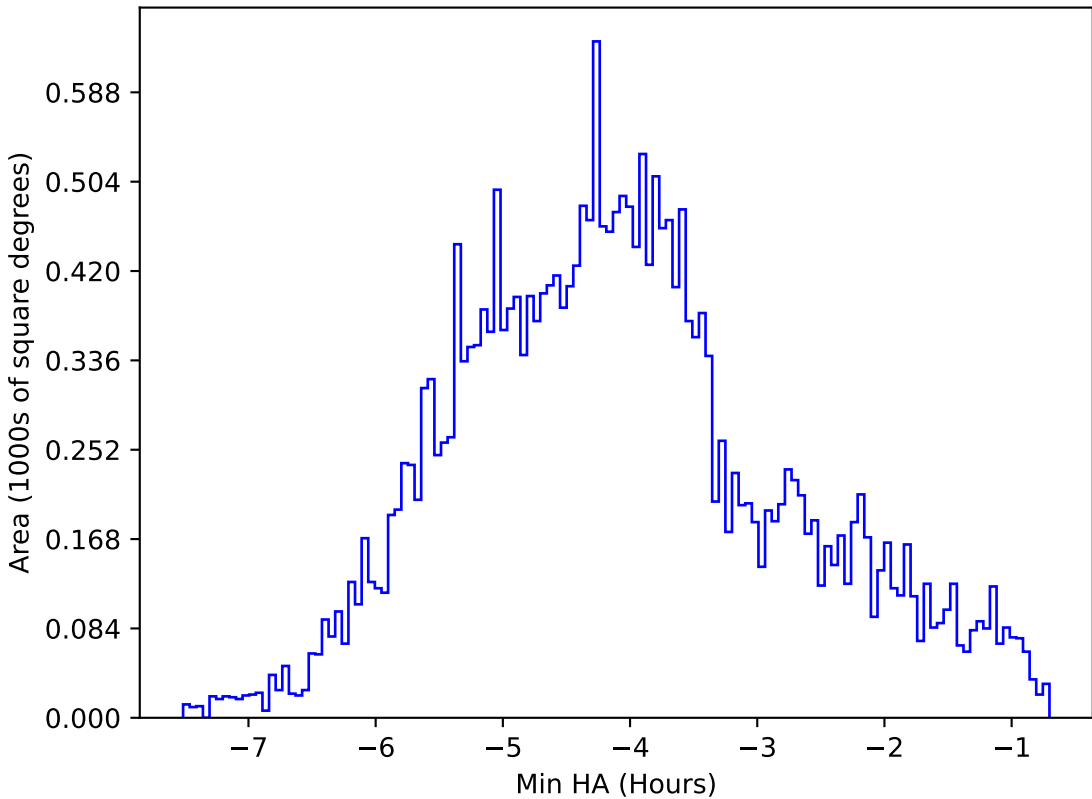
too_elab_r16_d2_griz_v3.4_10yrs All sky z band: Min HA
