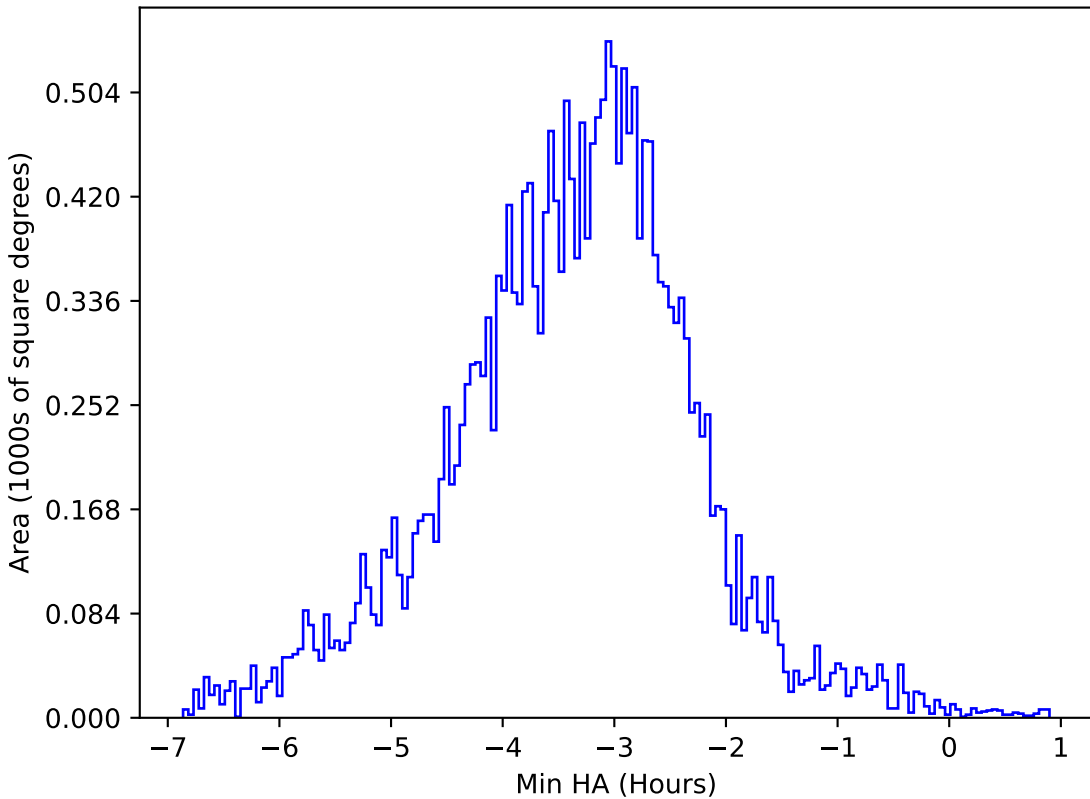
too_elab_r16_d2_griz_v3.4_10yrs All sky y band: Min HA
