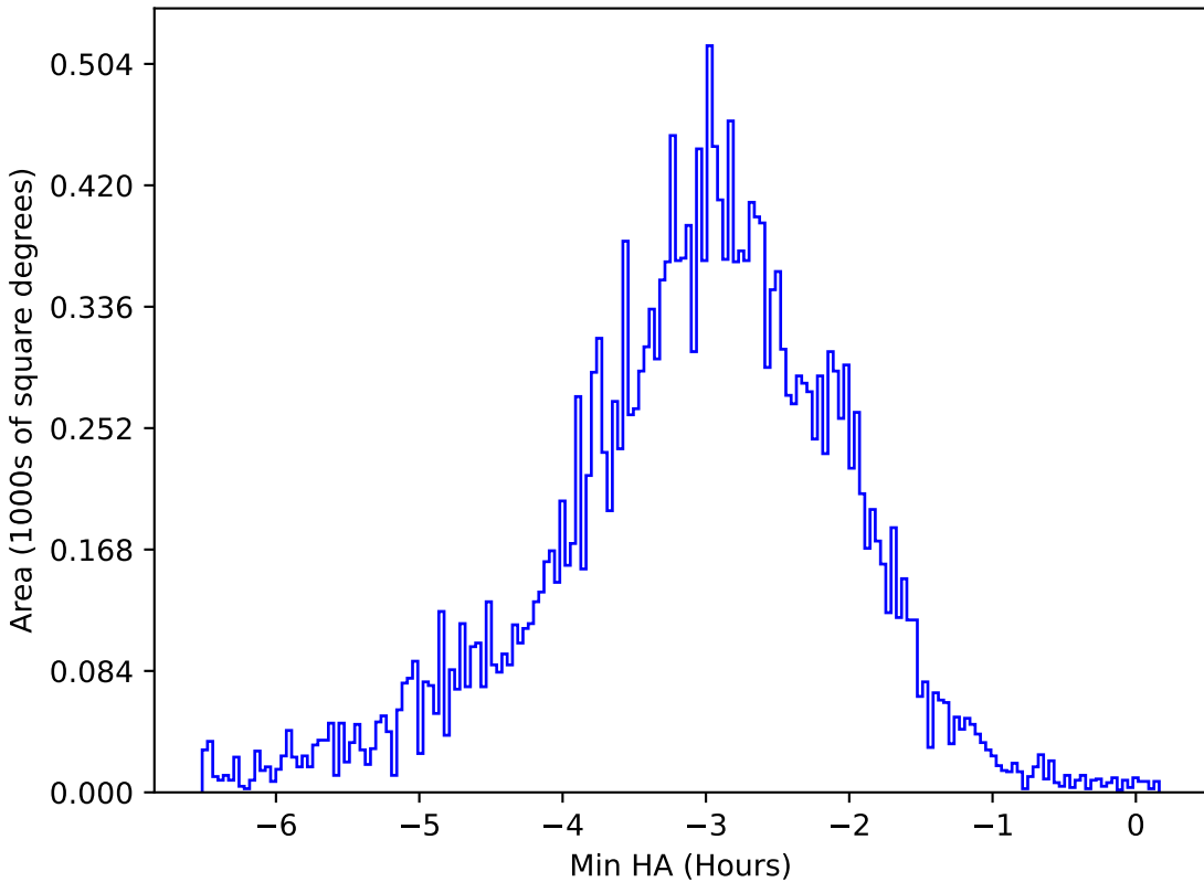
too_elab_r16_d2_griz_v3.4_10yrs All sky u band: Min HA
