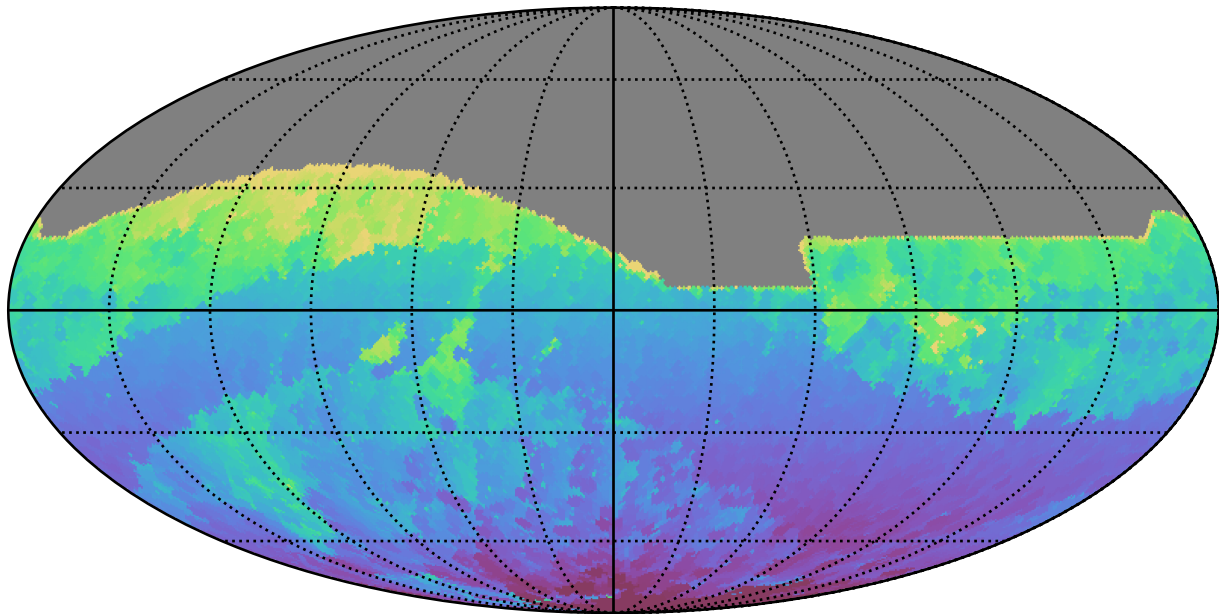
too_elab_r16_d2_griz_v3.4_10yrs All sky r band: Min HA
