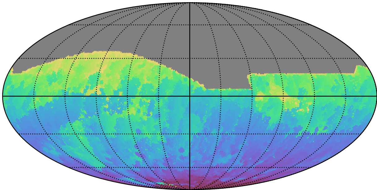
too_elab_r16_d2_griz_v3.4_10yrs All sky i band: Min HA
