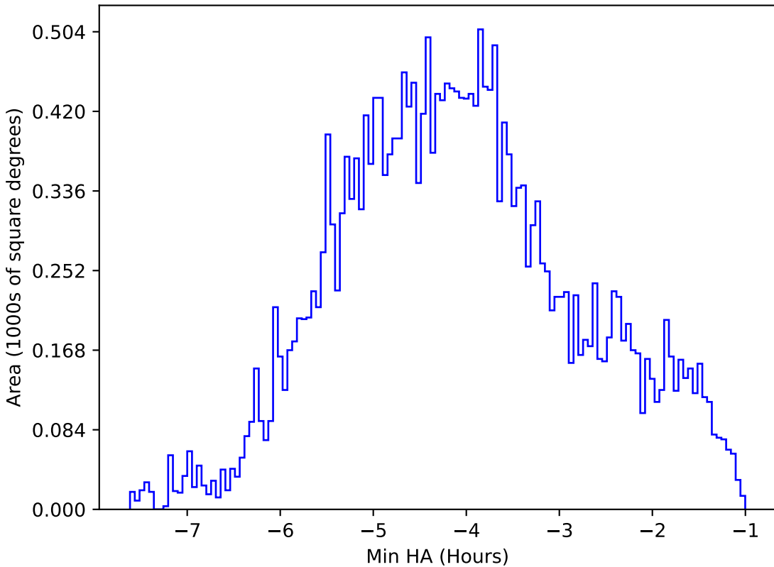
too_elab_r16_d2_griz_v3.4_10yrs All sky i band: Min HA
