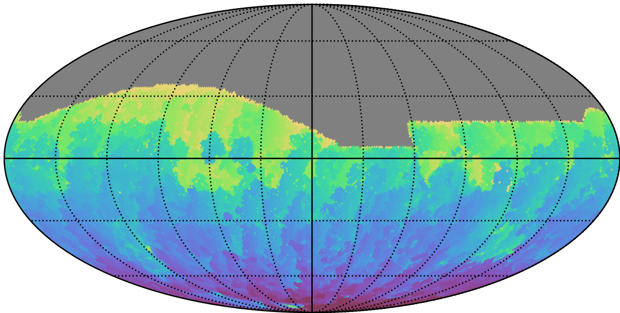
too_elab_r16_d2_griz_v3.4_10yrs All sky g band: Min HA
