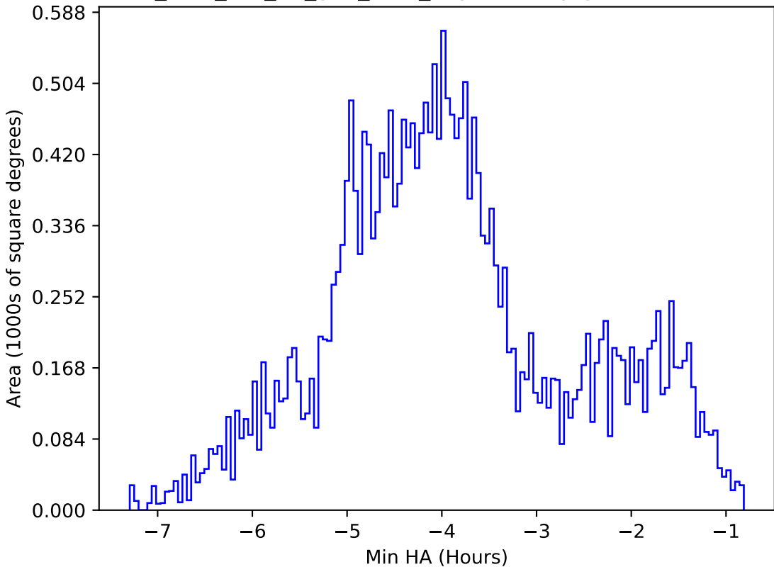
too_elab_r16_d2_griz_v3.4_10yrs All sky g band: Min HA
