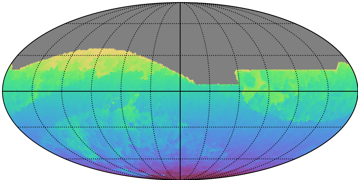
too_elab_r16_d2_griz_v3.4_10yrs All sky all bands: Min HA
