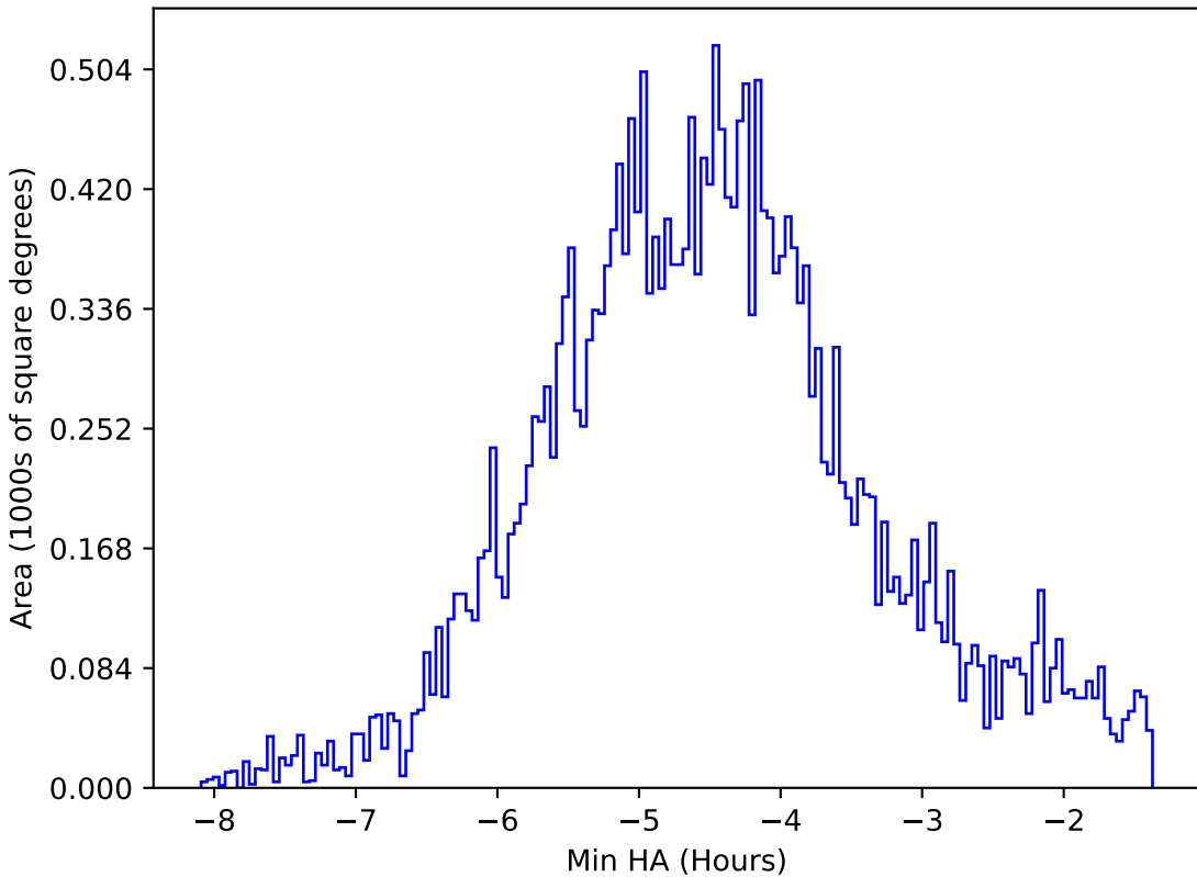
too_elab_r16_d2_griz_v3.4_10yrs All sky all bands: Min HA
