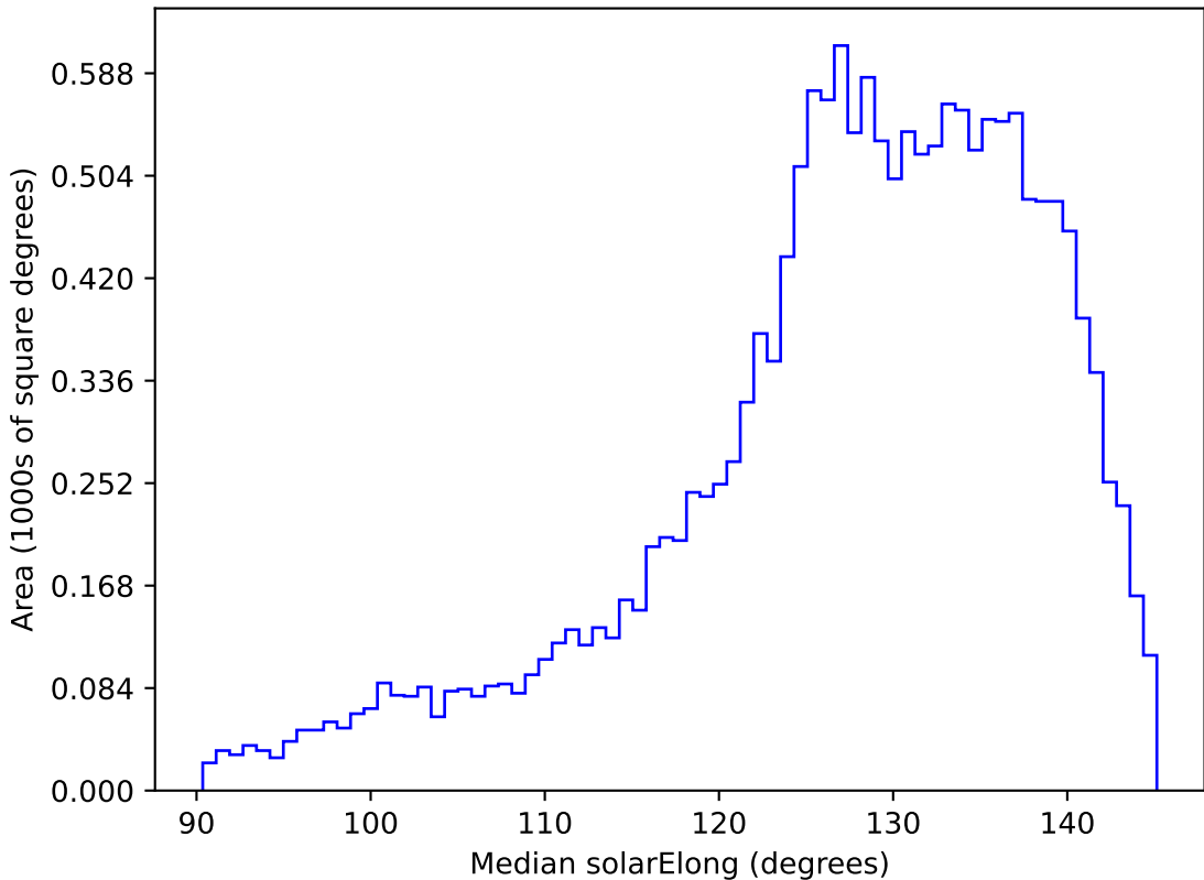
too_elab_r16_d2_griz_v3.4_10yrs WFD z band: Median solarElong
