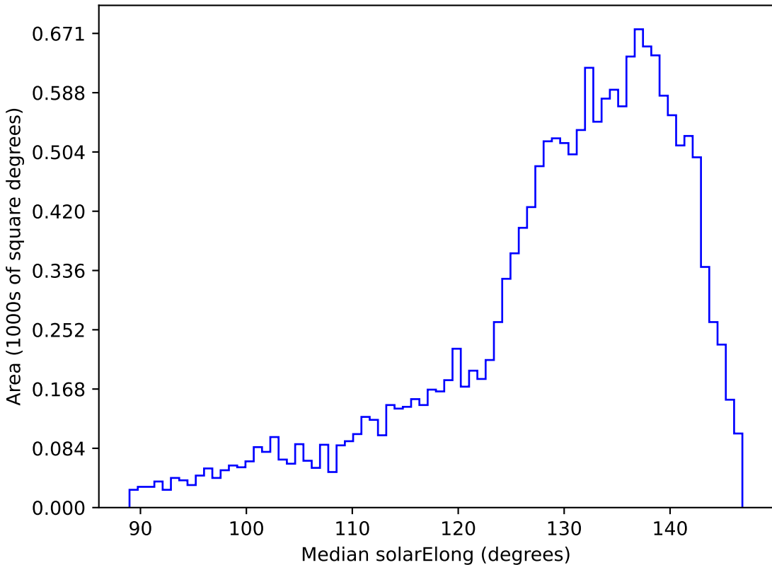
too_elab_r16_d2_griz_v3.4_10yrs WFD y band: Median solarElong
