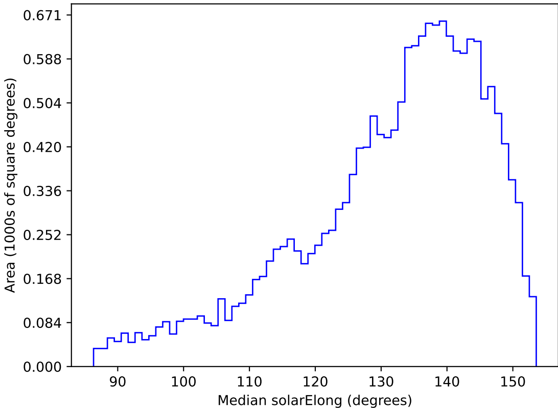
too_elab_r16_d2_griz_v3.4_10yrs WFD u band: Median solarElong
