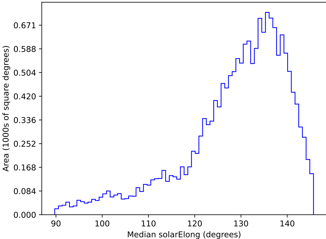
too_elab_r16_d2_griz_v3.4_10yrs WFD i band: Median solarElong
