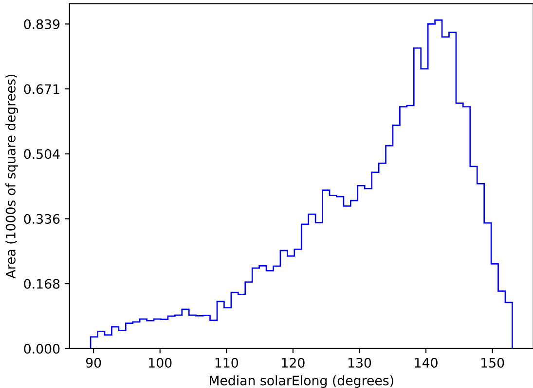
too_elab_r16_d2_griz_v3.4_10yrs WFD g band: Median solarElong
