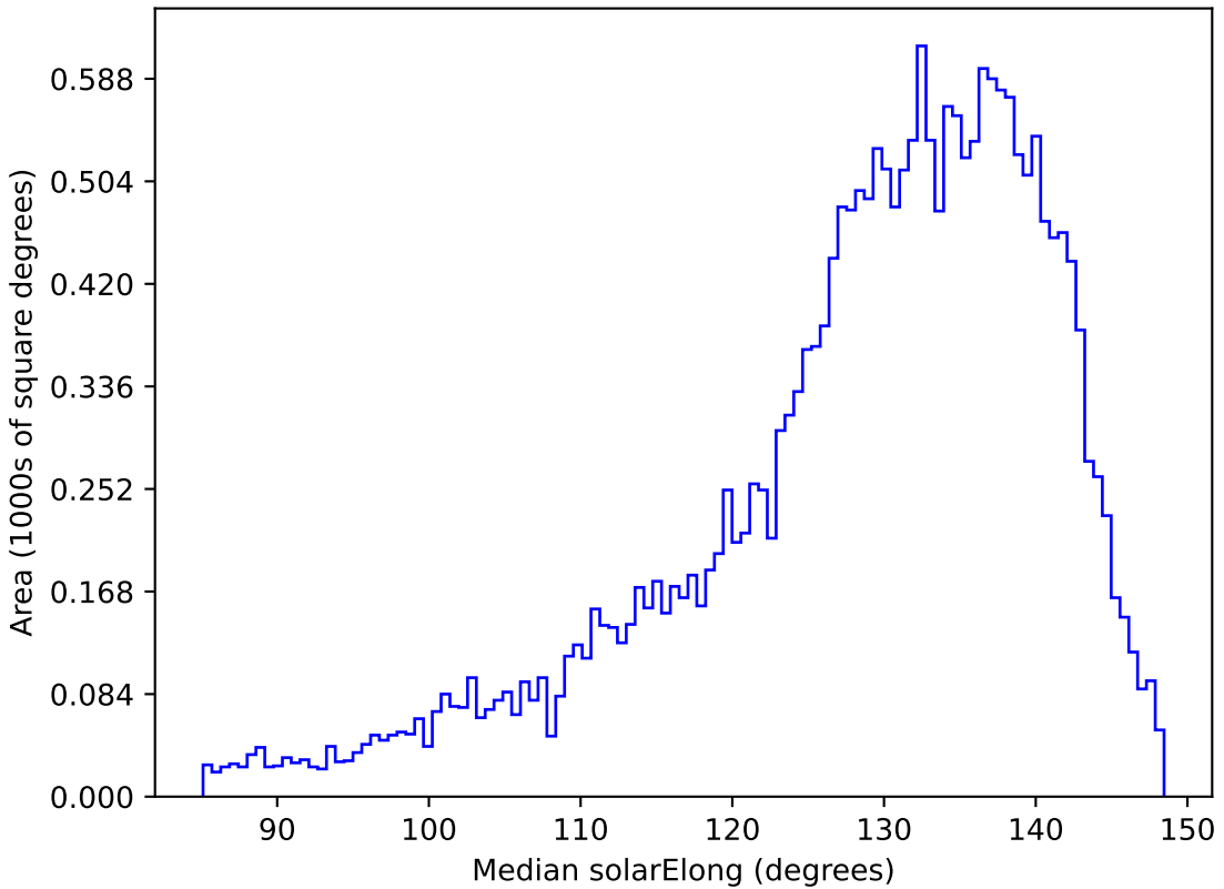
too_elab_r16_d2_griz_v3.4_10yrs All sky y band: Median solarElong
