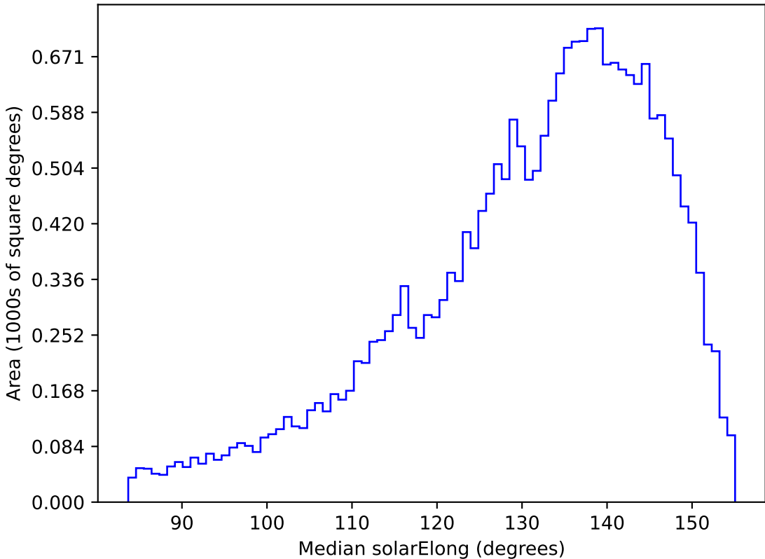
too_elab_r16_d2_griz_v3.4_10yrs All sky u band: Median solarElong
