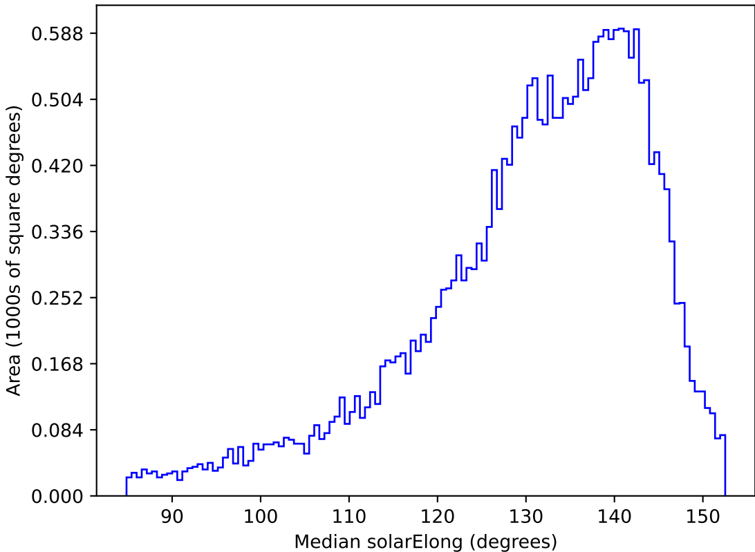
too_elab_r16_d2_griz_v3.4_10yrs All sky r band: Median solarElong
