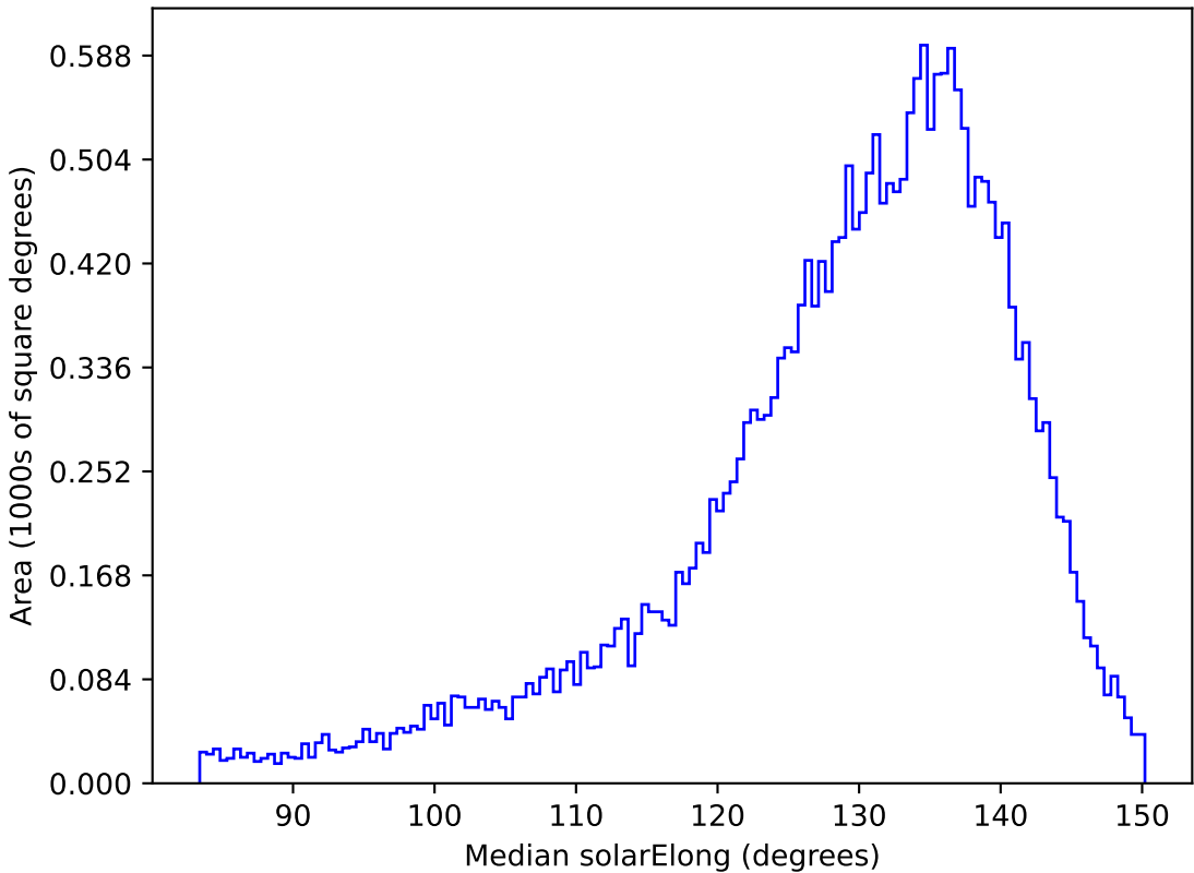
too_elab_r16_d2_griz_v3.4_10yrs All sky i band: Median solarElong
