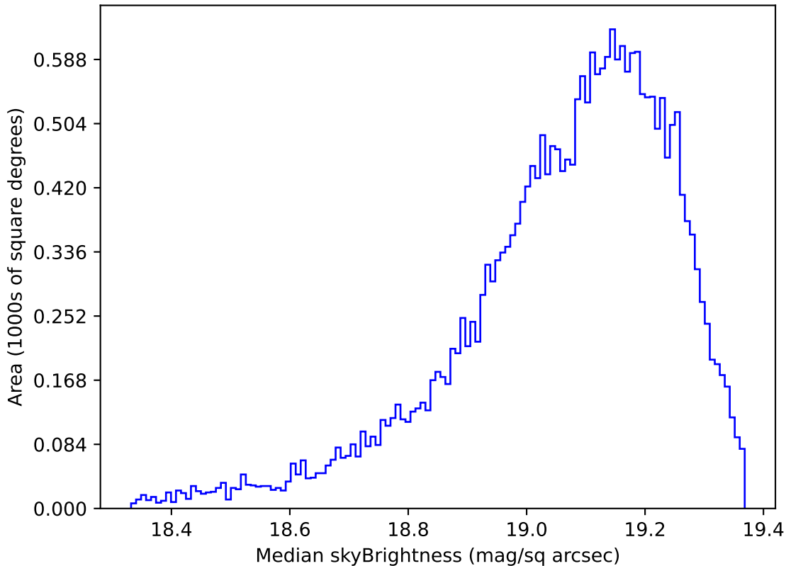
too_elab_r16_d2_griz_v3.4_10yrs Yr 1 z band: Median skyBrightness
