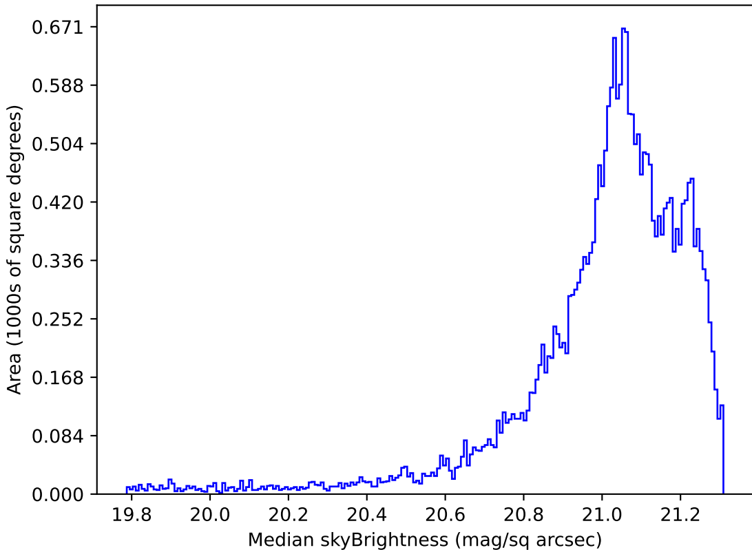
too_elab_r16_d2_griz_v3.4_10yrs Yr 1 r band: Median skyBrightness
