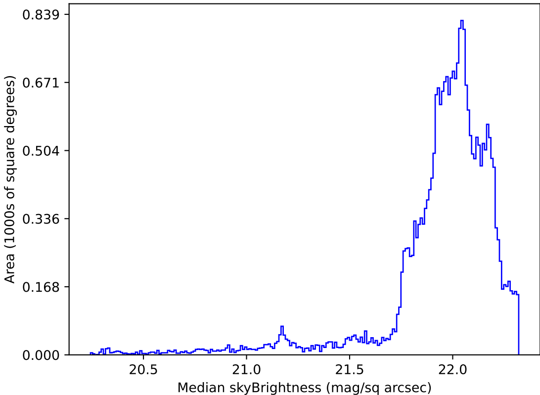
too_elab_r16_d2_griz_v3.4_10yrs Yr 1 g band: Median skyBrightness
