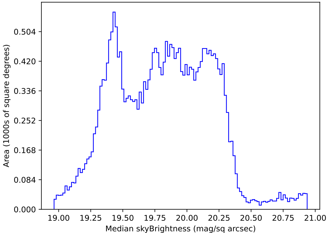
too_elab_r16_d2_griz_v3.4_10yrs Yr 1 all bands: Median skyBrightness
