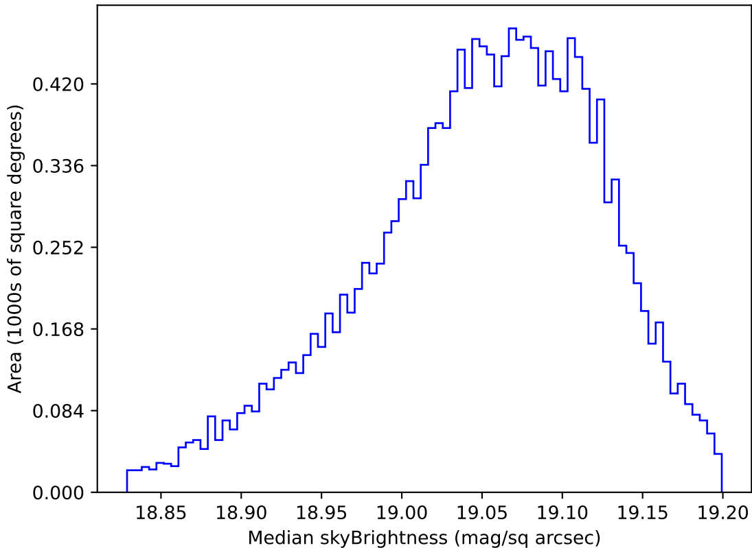
too_elab_r16_d2_griz_v3.4_10yrs WFD z band: Median skyBrightness
