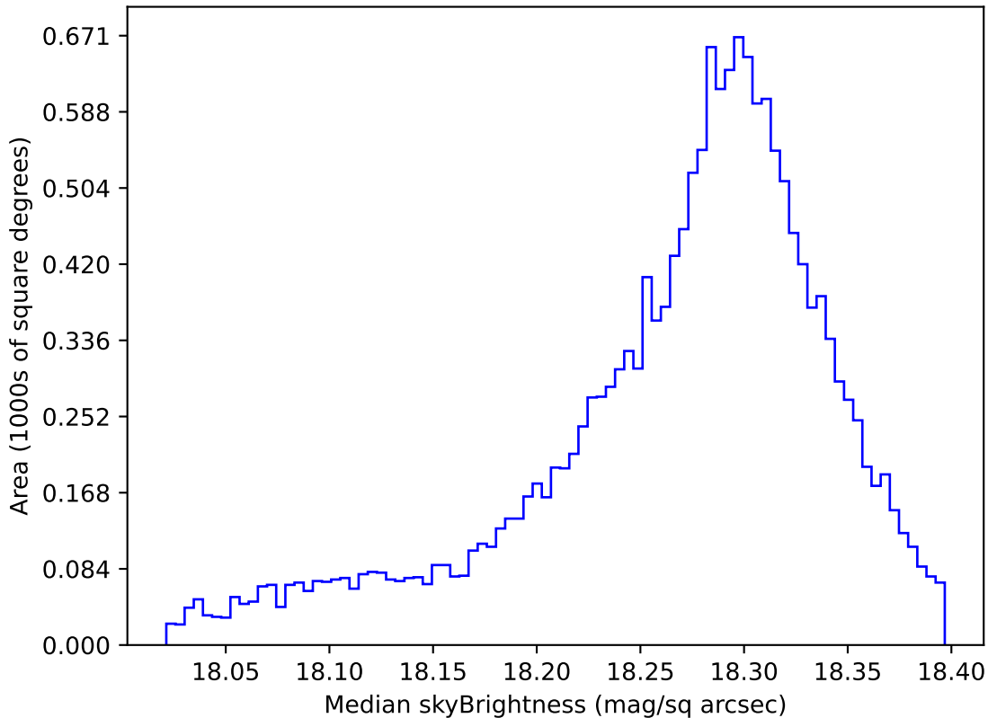
too_elab_r16_d2_griz_v3.4_10yrs WFD y band: Median skyBrightness
