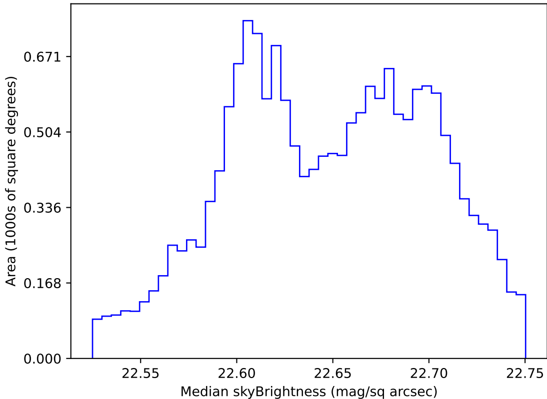
too_elab_r16_d2_griz_v3.4_10yrs WFD u band: Median skyBrightness
