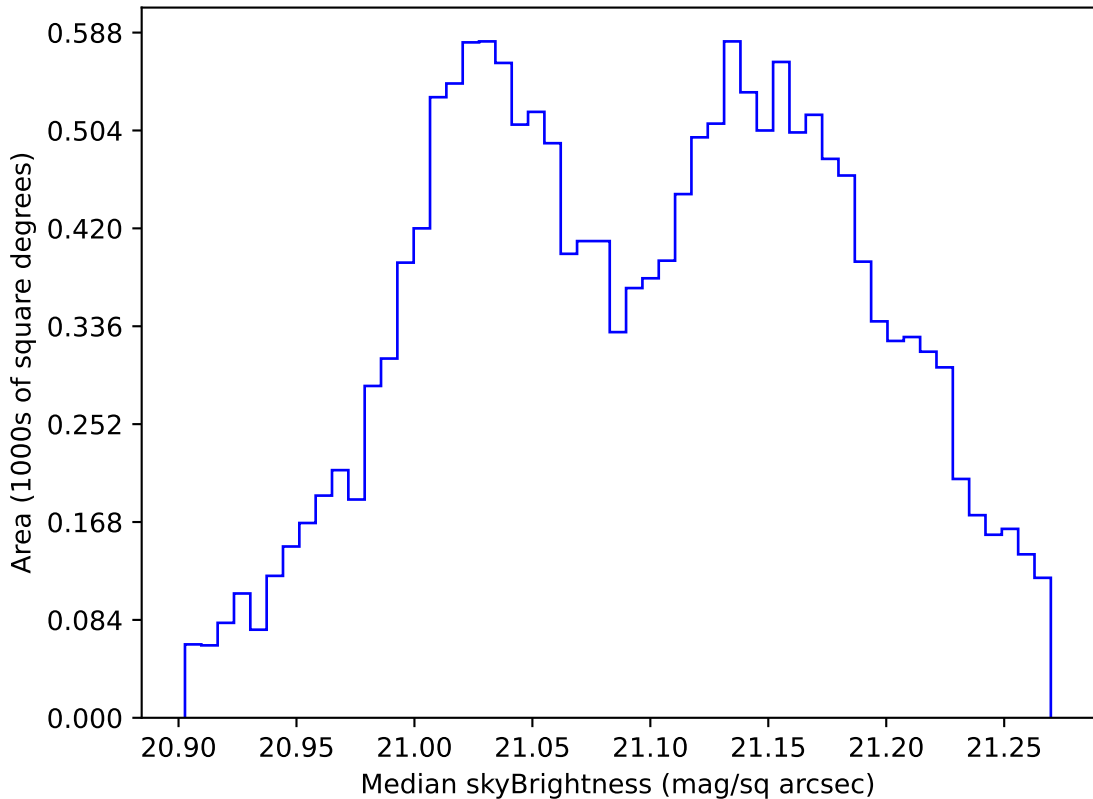
too_elab_r16_d2_griz_v3.4_10yrs WFD r band: Median skyBrightness
