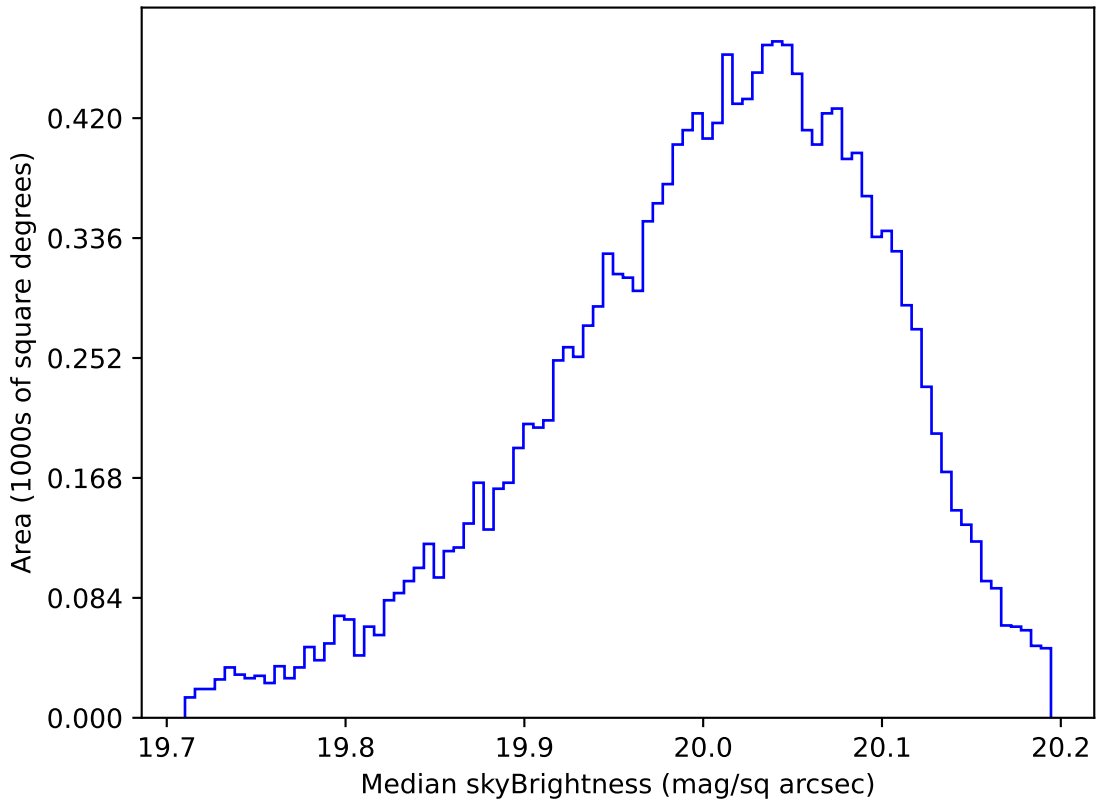
too_elab_r16_d2_griz_v3.4_10yrs WFD i band: Median skyBrightness
