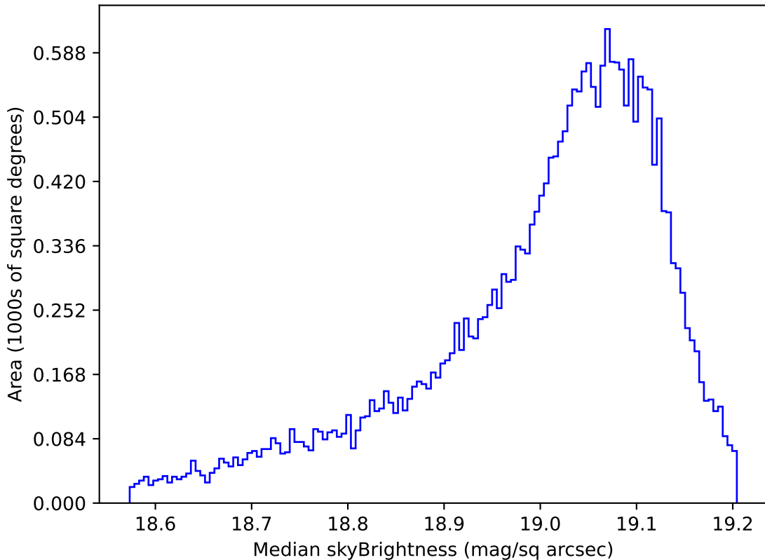
too_elab_r16_d2_griz_v3.4_10yrs All sky z band: Median skyBrightness
