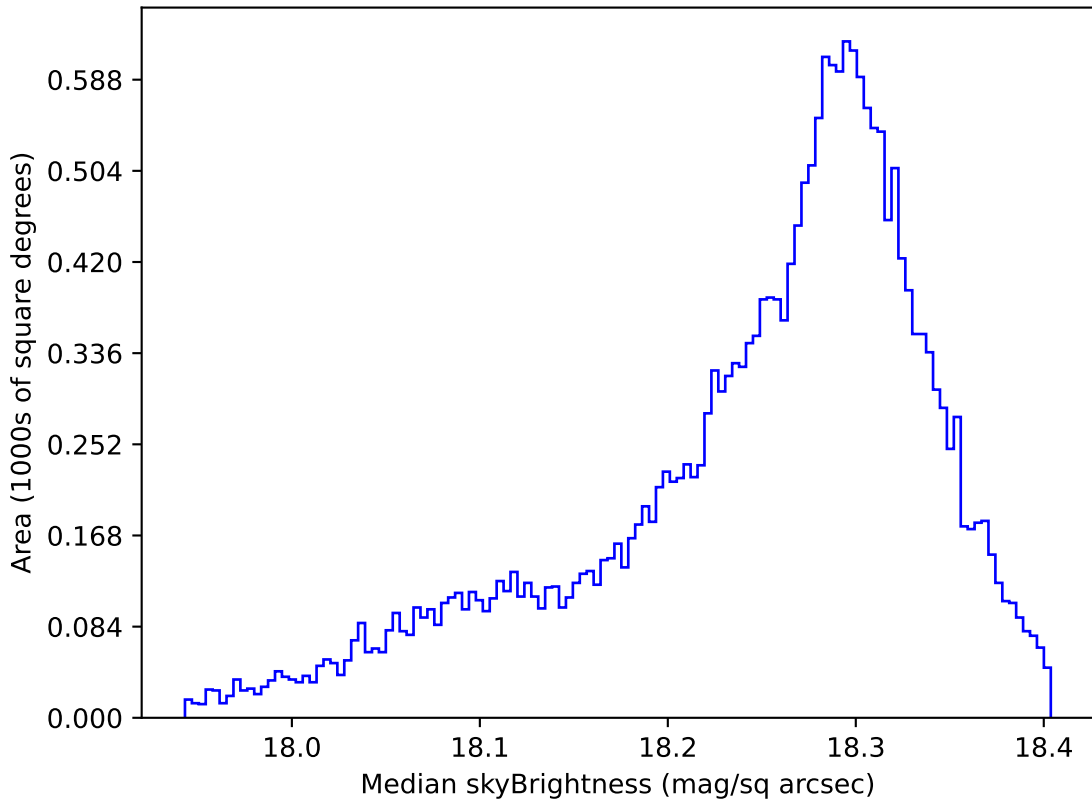
too_elab_r16_d2_griz_v3.4_10yrs All sky y band: Median skyBrightness
