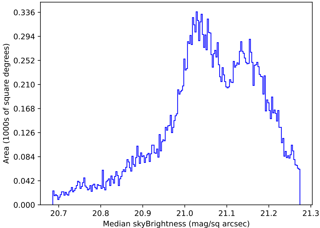
too_elab_r16_d2_griz_v3.4_10yrs All sky r band: Median skyBrightness
