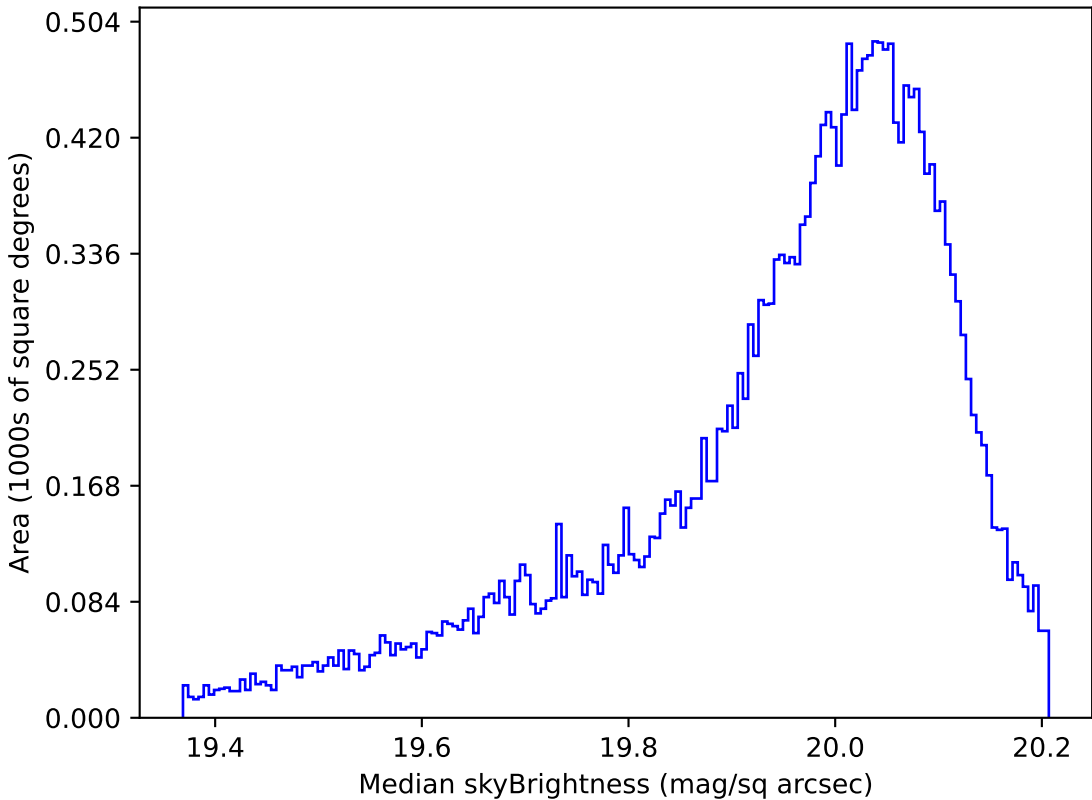
too_elab_r16_d2_griz_v3.4_10yrs All sky i band: Median skyBrightness
